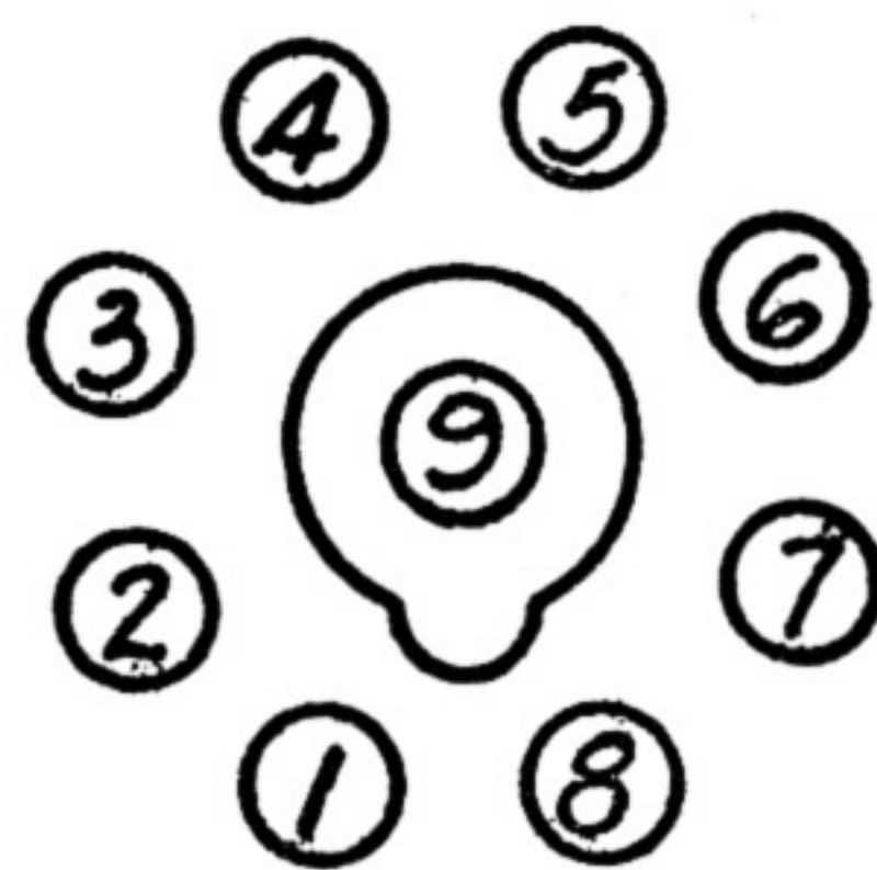
BOTTOM VIEW OF SOCKET
